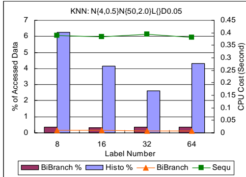
Figure 12: Sensitivity to Number of Labels in Trees for k -NN Queries
