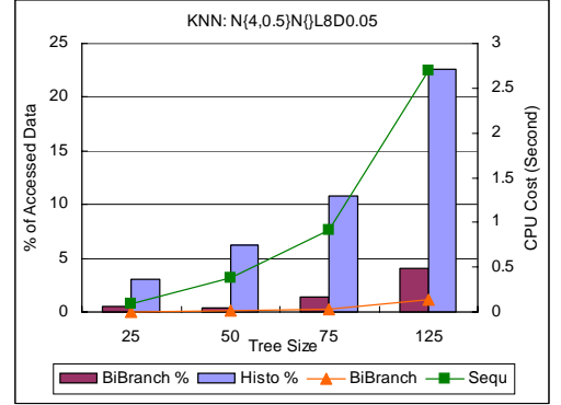
Figure 10: Sensitivity to Size of Trees for k -NN Queries
